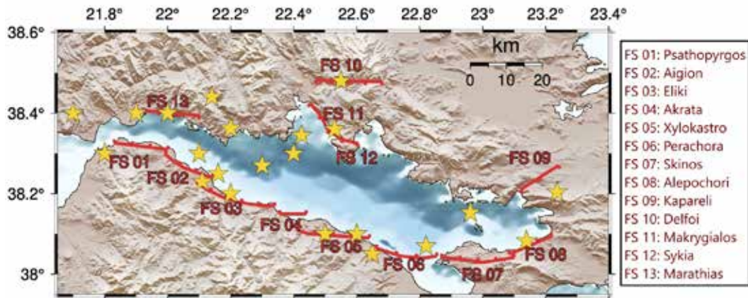
Figure 1. Geomorphological map of Corinth Rift, where the major normal fault segments are represented by red solid lines. Yellow stars depict the M \geq 6.0 earthquakes occurred in the study area since 1714.
