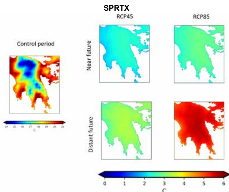
Figure 1. Absolute differences of spring (April-May) maximum temperature, between the reference period and the near or distant for two climate scenarios (RCP4.5, RCP8.5)
