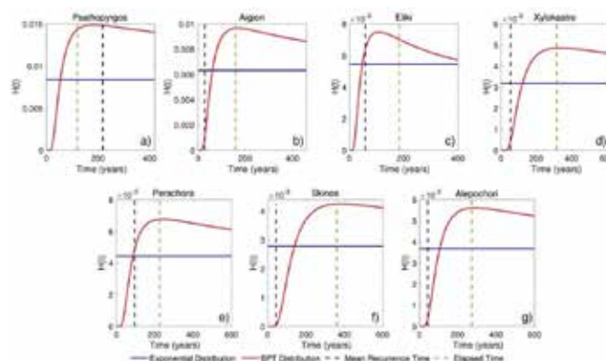
Figure 3. Hazard functions, H(t) , for the Psathopyrgos (a), Aigion (b), Eliki (c), Xylokastro (d), Perachora (e), Skinos (f) and Alepochori (g) fault segments according to the Exponential (blue solid lines) and the BPT (solid red lines) distributions. Vertical dashed lines denote the elapsed time since the last M \geq 6.0 earthquake ( t = 0 ) occurred on each fault segment, whereas the vertical dashed black lines denote the mean recurrence time of M \geq 6.0 earthquake for each fault segment.
