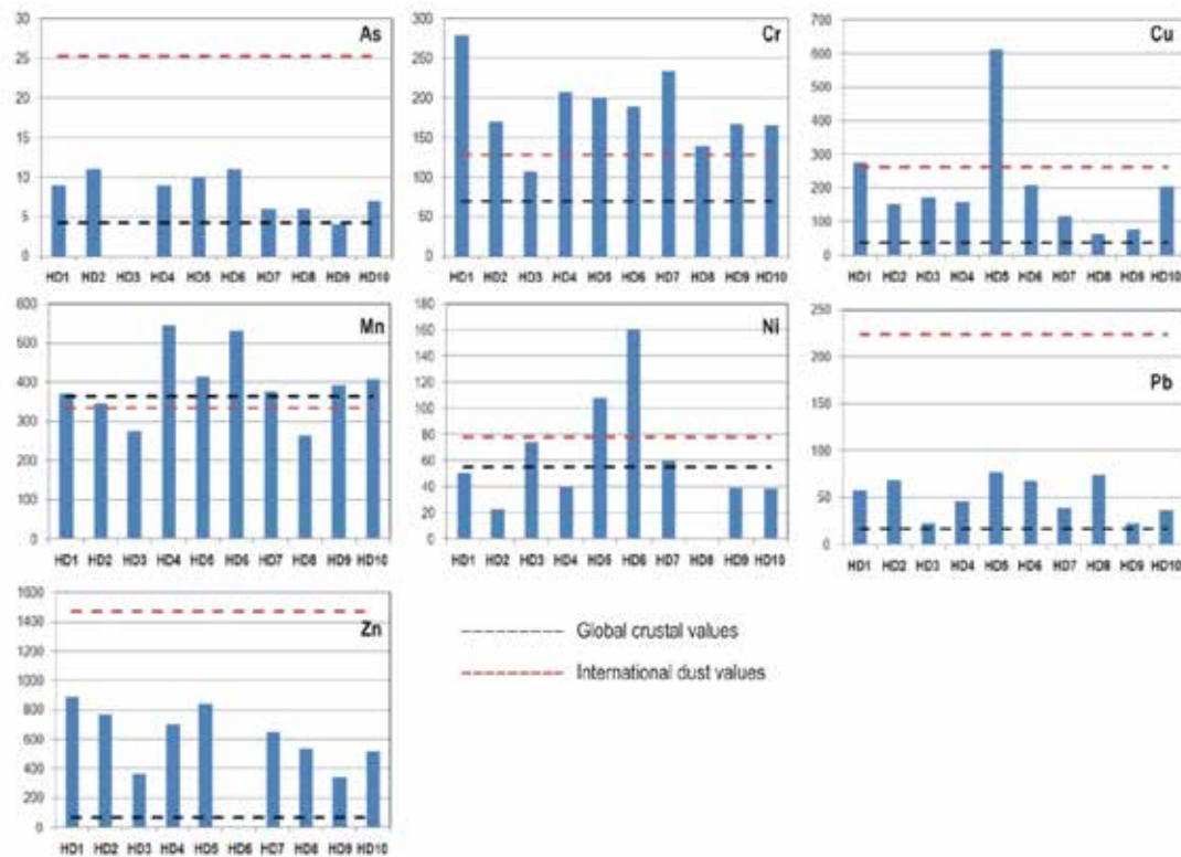
Figure 2. Heavy metal contents ( \text{mg kg}^{-1} ) in house dust samples. Global crustal elemental concentrations (black dashed line, data in Table 1) and international dust values (red dashed line, data in Table 1).
